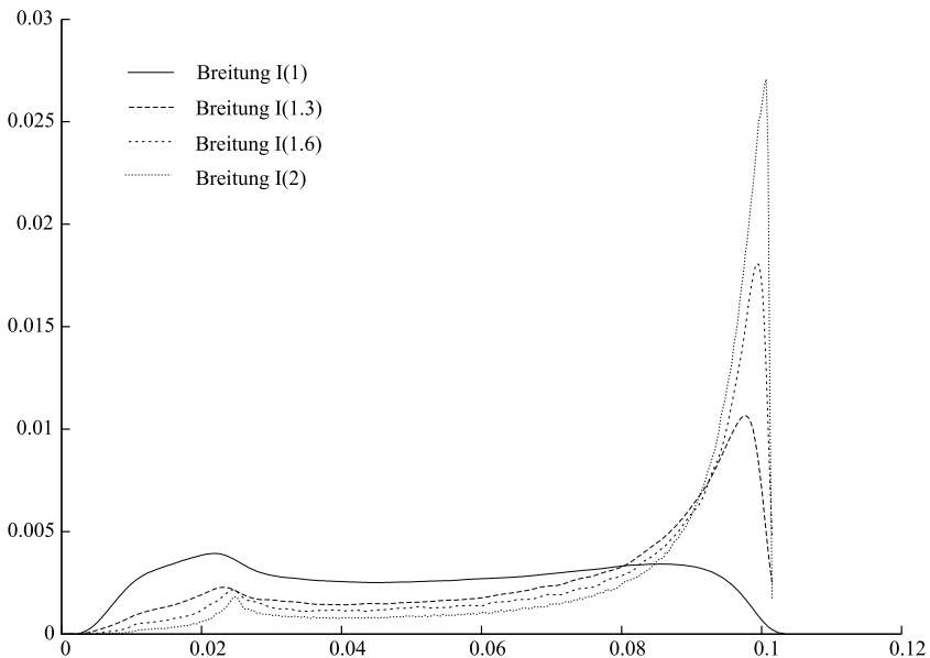
FIGURE 1. Kernel density plots of Breitung’s statistic computed from one million replications of I(d) series ( n = 1,000 ).
